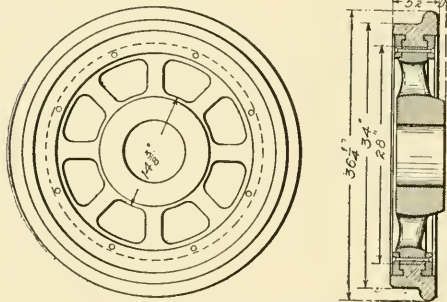
Fig. 24. Steel-Tired Wheel
